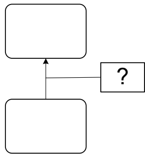
Causality: If...then
