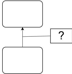
Causality: If...then
